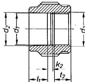
Type MGI Socket with internal thread at one end (reinforced)
