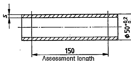
Figure 1. Test piece
