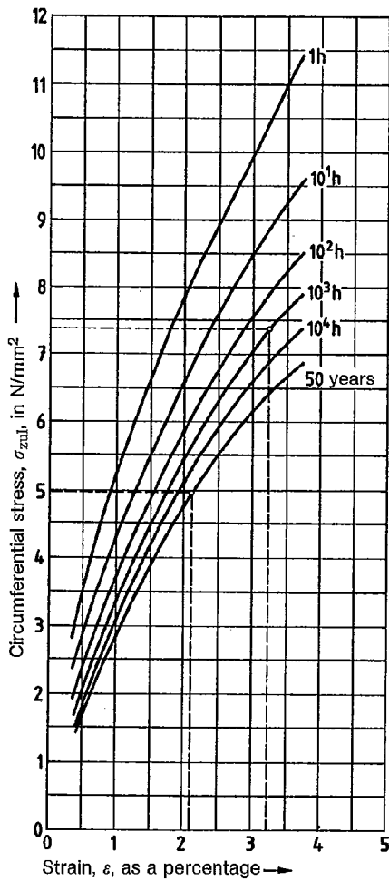
Figure 2. Stress-strain diagram for PE-HD at 20°C
