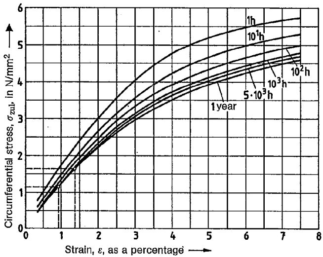
Figure 4. Stress-strain diagram for PE-HD at 80°C
