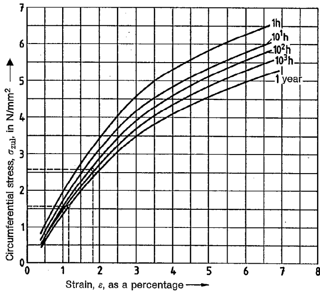
Figure 3. Stress-strain diagram for PE-HD at 70°C
